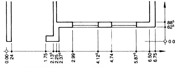
4 Dimensions given by coordinates (drawn at 1:50 cm, m; units = cm and m)
